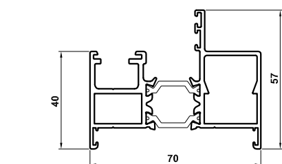
Contemporary ETD017 Outer Frame
