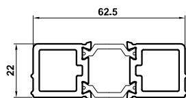
ETD052 Outer Frame Coupler
