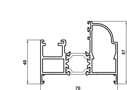
Classic-al ETD015 Outer Frame
