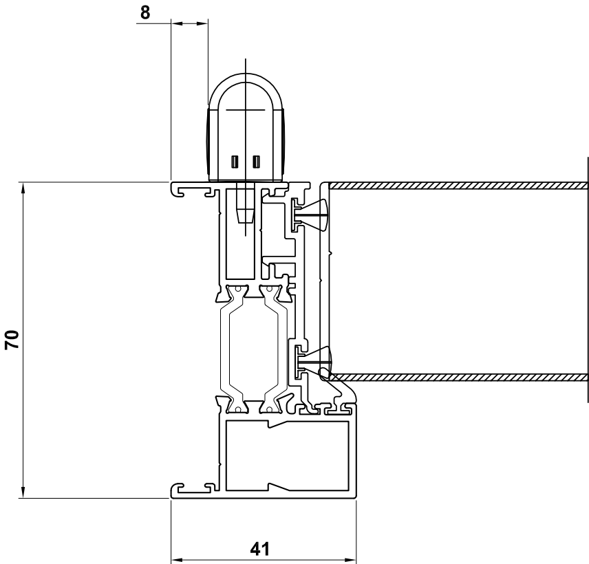
Contemporary Frame
